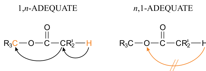
Fig. 5: Schematic correlations in an O-acetyl group ( R' = H ) attached to a quaternary carbon atom ( R \neq H ) for an 1, n - and n ,1-ADEQUATE experiment. The 1, n -ADEQUATE experiment allows to observe a correlation from the protons of the methyl group to the quaternary carbon atom. For the n ,1-ADEQUATE experiment no correlation is expected in this case because the first transfer ( ^3J_{CH} HMBC) would end at an oxygen atom.
